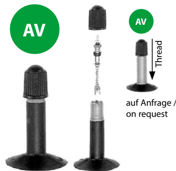
AUTO/SCHRADER/AMERICAN 35/40/48 mm
